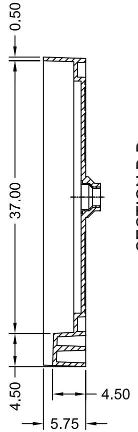
SECTION B-B
